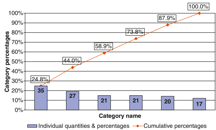
Fig. 4.5 Pareto chart.
